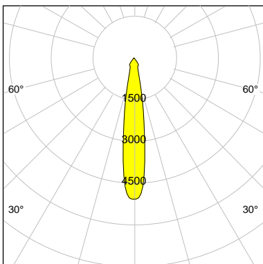
I-max : 5072 cd/klm *
