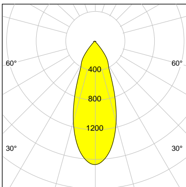
I-max : 1670 cd/klm *
