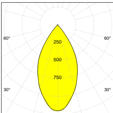
I-max : 1203 cd/klm *
